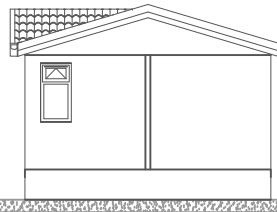
Elevation D
